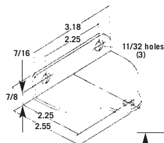
MOUNTING BRACKET
